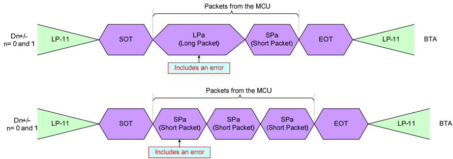
Figure 81 Errors Packets
